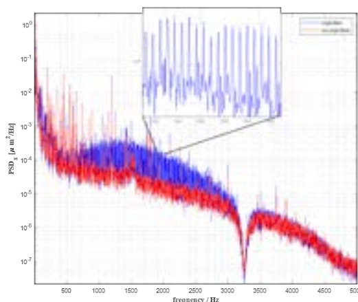
Figure 4: Horizontal power spectral density, derived from the FA data path at 10 kHz sampling rate. The blue curve was recorded under standard operational conditions. The detail enlargement shows a series of frequency lines equally spaced by 6.25 Hz. This frequency is characteristic for the top-up injection in PETRA III. For the red curve the injection was gated-out.
